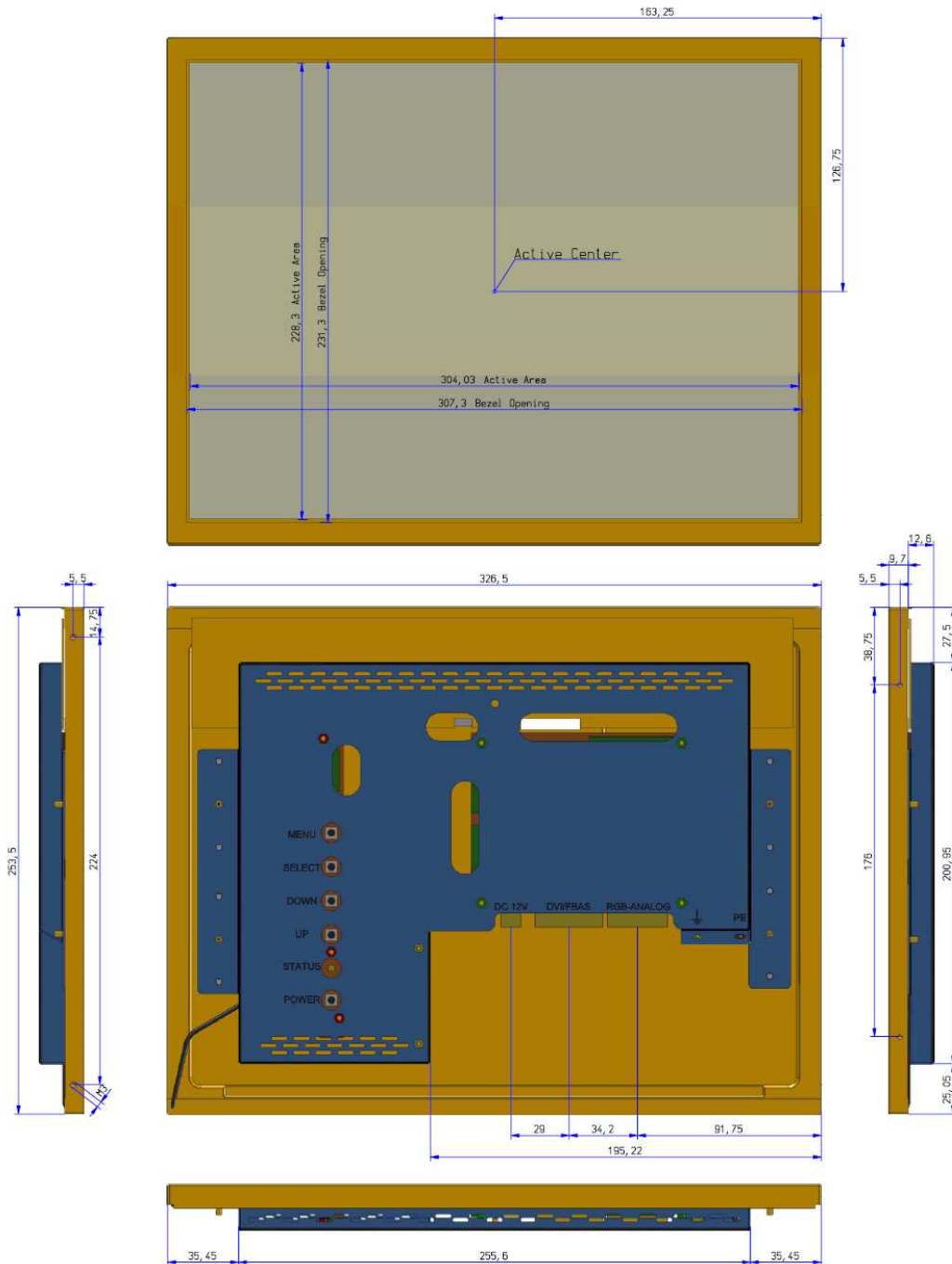
Figure 1: Mechanical Outlines
