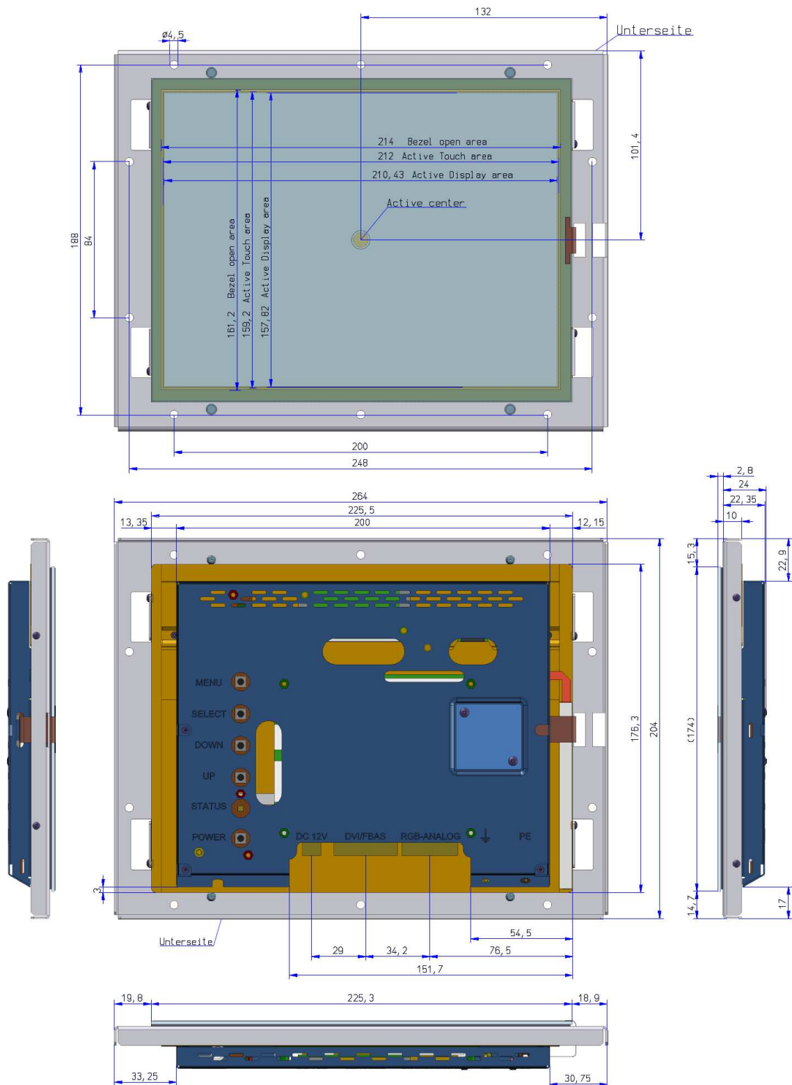
Figure 1: Mechanical Outlines
