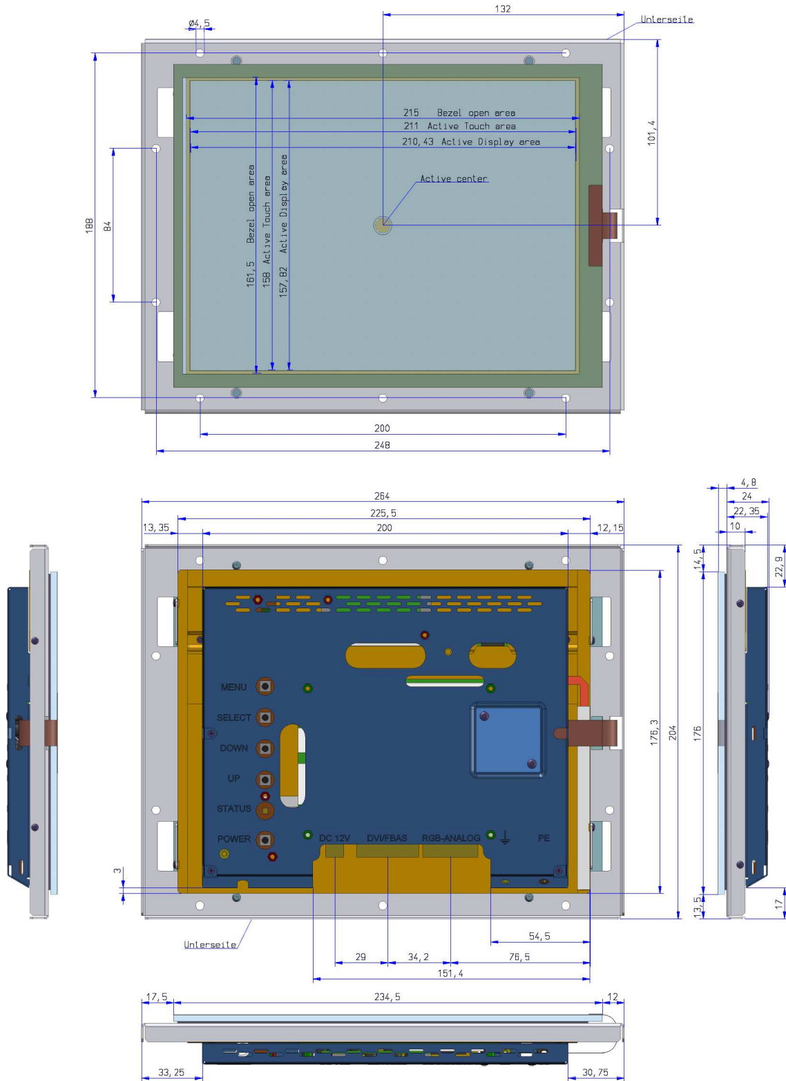
Figure 1: Mechanical Outlines
