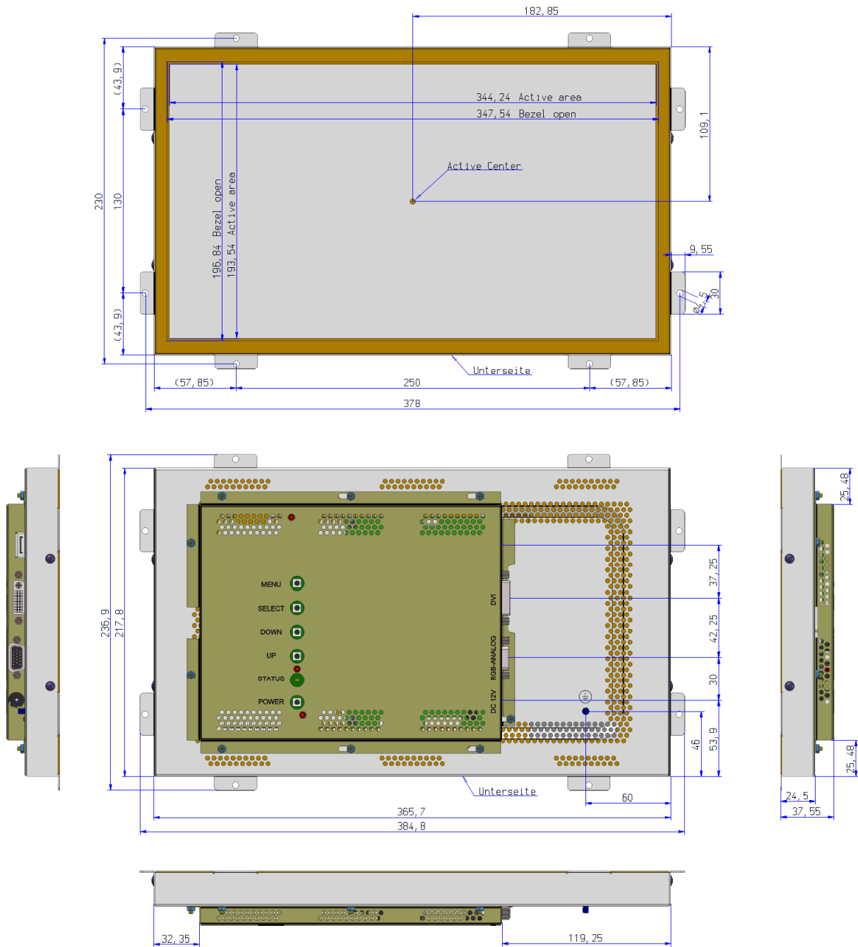
Figure 1: Mechanical Outlines
