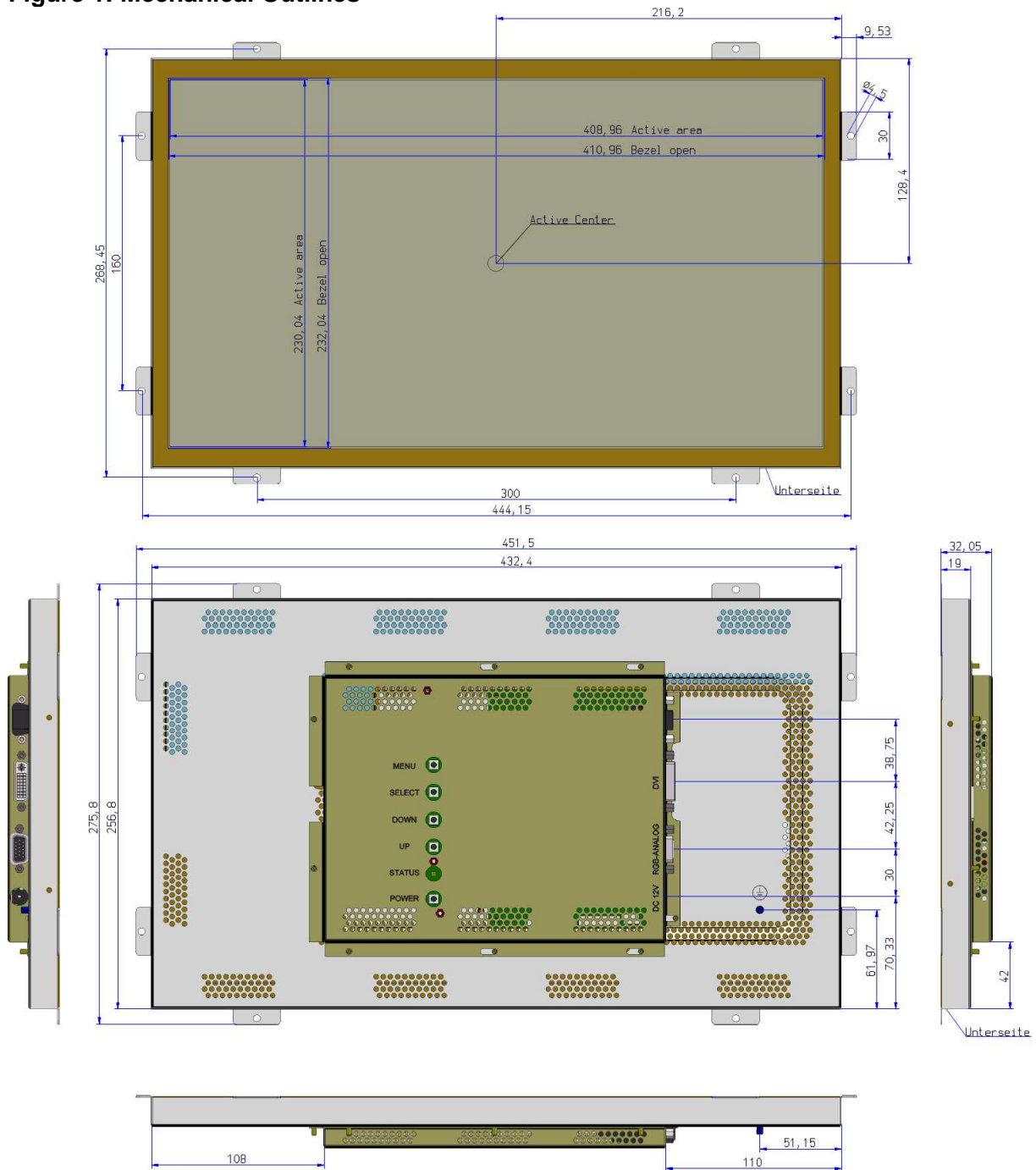
Figure 1: Mechanical Outlines
