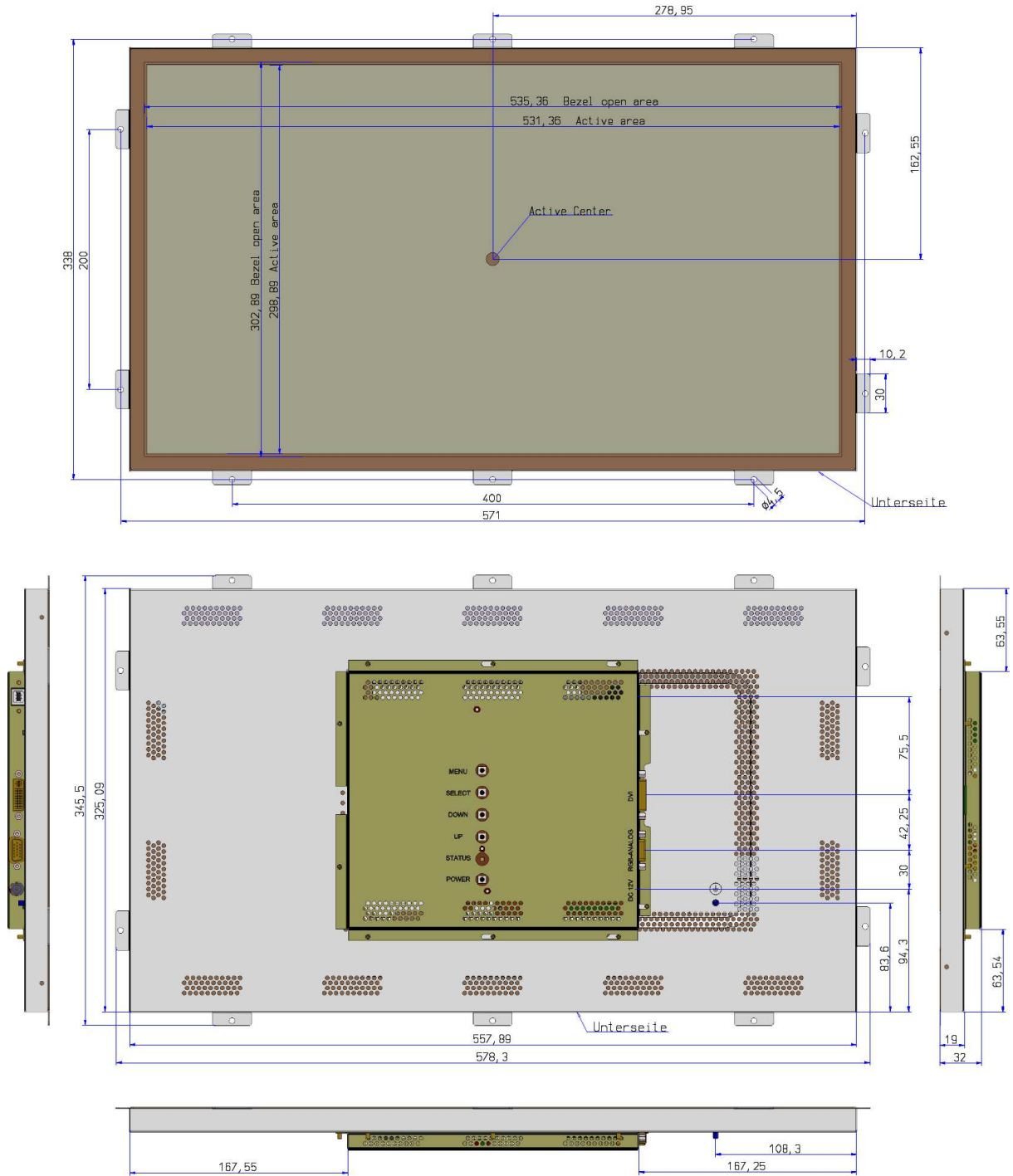
Figure 1: Mechanical Outlines
