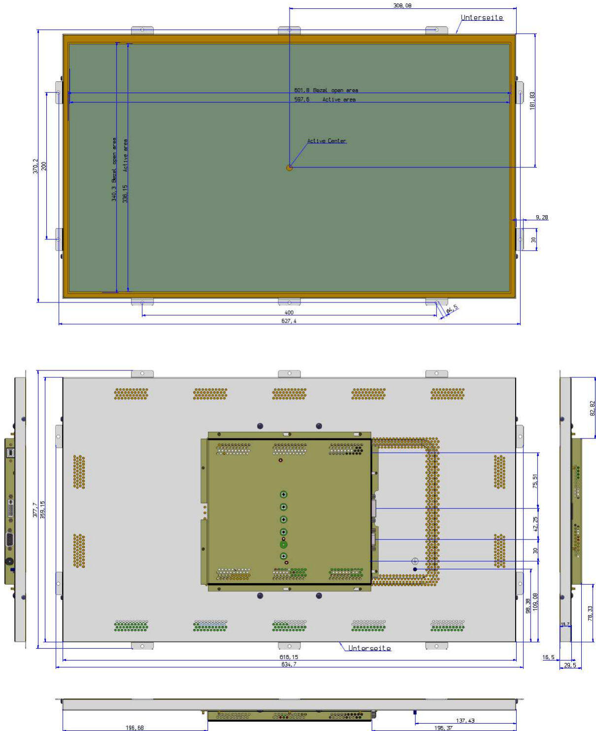
Figure 1: Mechanical Outlines
