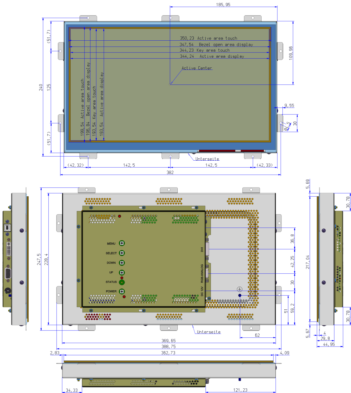
Figure 1: Mechanical Outlines
