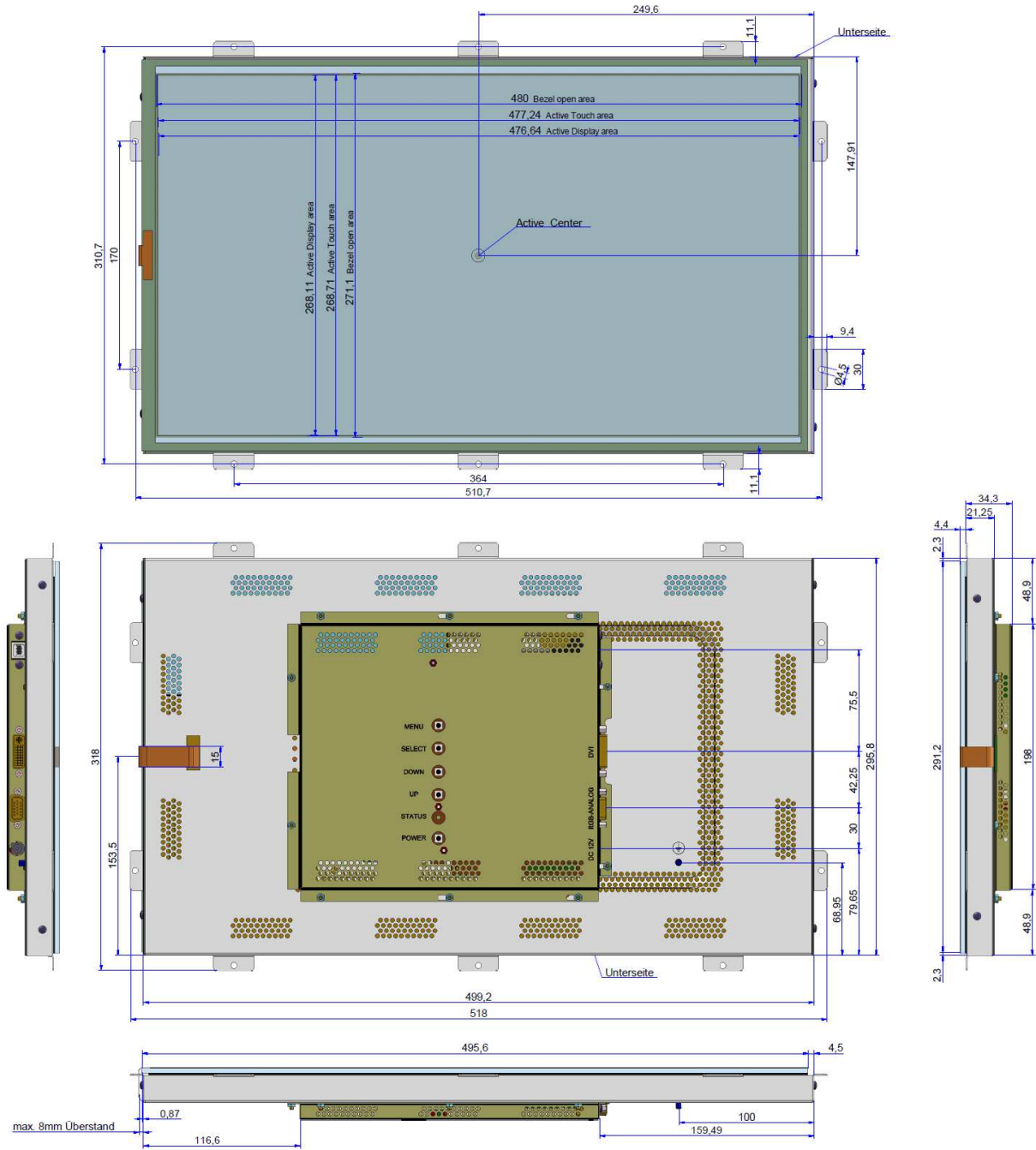
Figure 1: Mechanical Outlines
