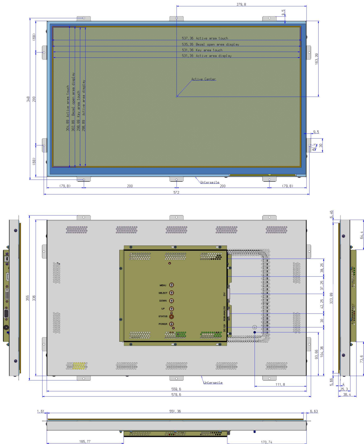
Figure 1: Mechanical Outlines
