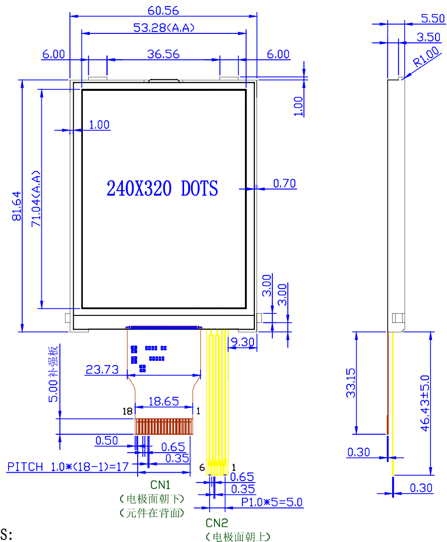
CN2 (LED)
